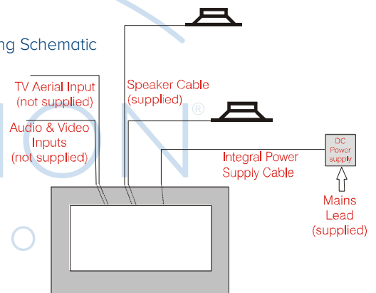
Fig 2. Installation Schematic:
