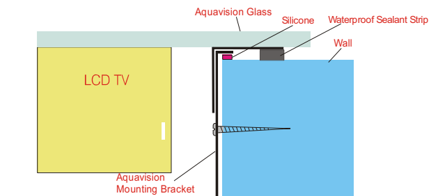
Fig 2. Installation Schematic:
